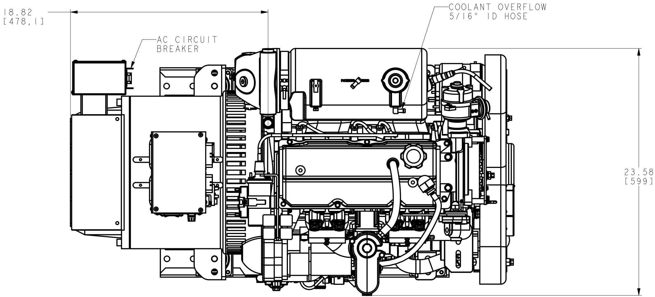
(TOP VIEW)
